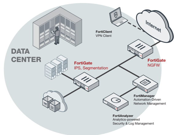
FortiGate 2000E deployment in data center (NGFW, IPS, and Intent-based Segmentation)
